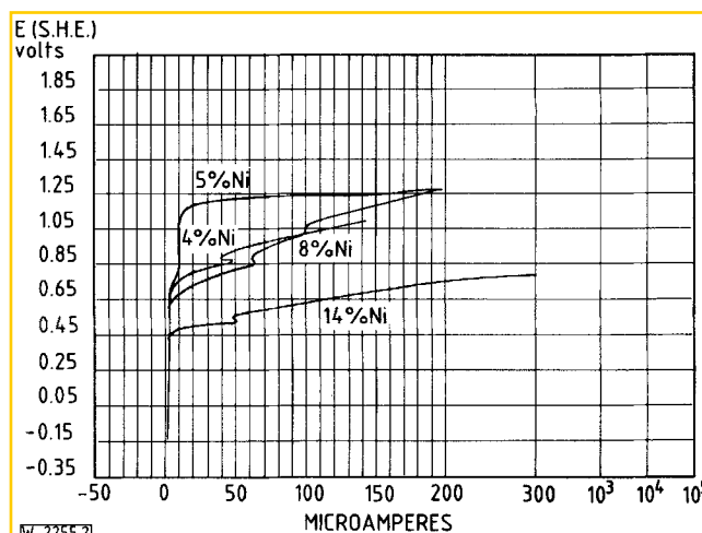
Fig. 2. Effect of increasing nickel, above the optimum, on the pitting potentials of duplex steels in 3% NaCl at 30°C
