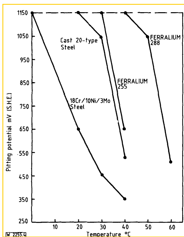
Fig. 4. Pitting potentials as a function of temperature
