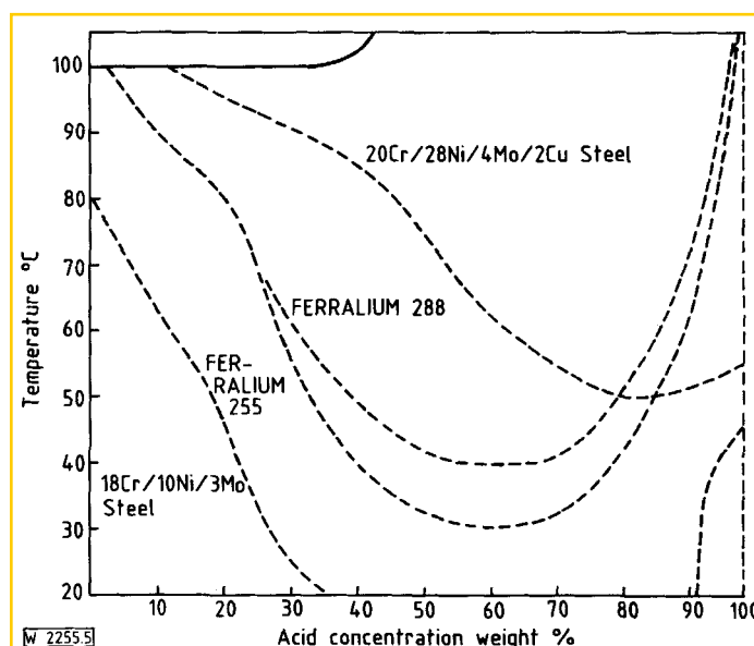
Fig. 5. Sulphuric acid corrosion chart based on maximum corrosion rate of 0.5 mm/year
